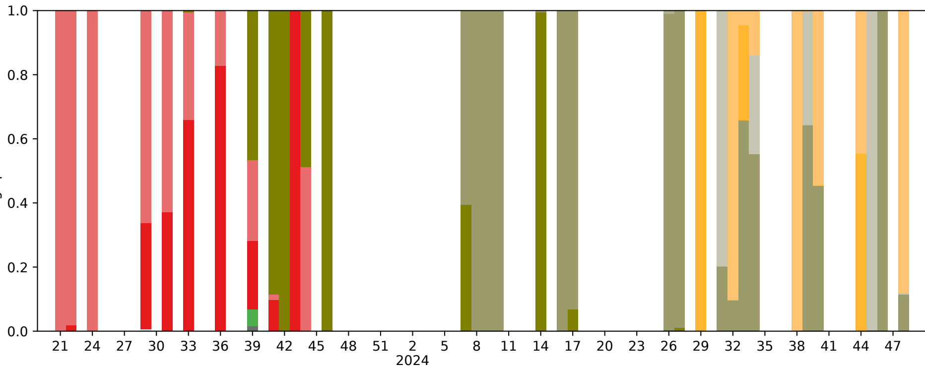
Lineage prevalence
